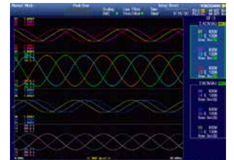
Eco-Mode Operation: Rated Speed, Rated Torque
